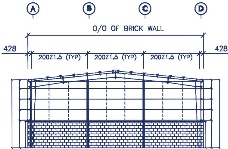
END WALL FRAMING HLE @ GL-6
