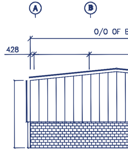
END WALL SHEETING HLE @ GL-6
