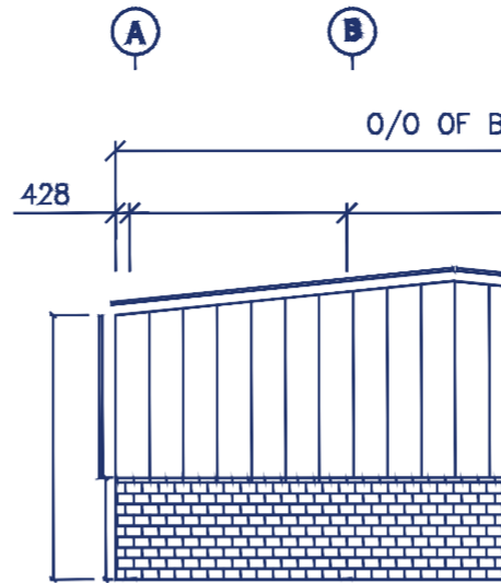
END WALL SHEETING HLE @ GL-1
