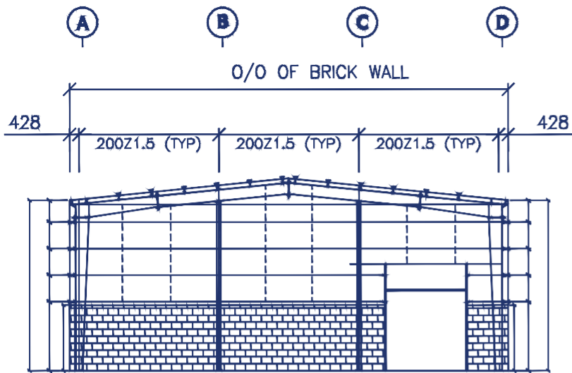
END WALL FRAMING HLE @ GL-1
